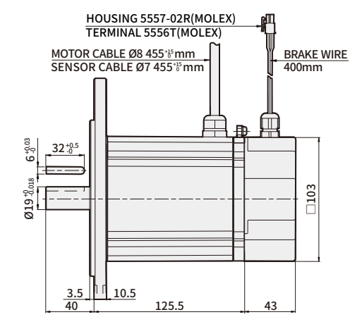
K20BK750NC-B (Brake type) Weight : 5.9Kg
