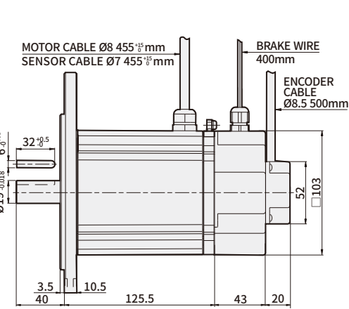
K20BK750NC-BE (Brake Encoder type) Weight : 6Kg
