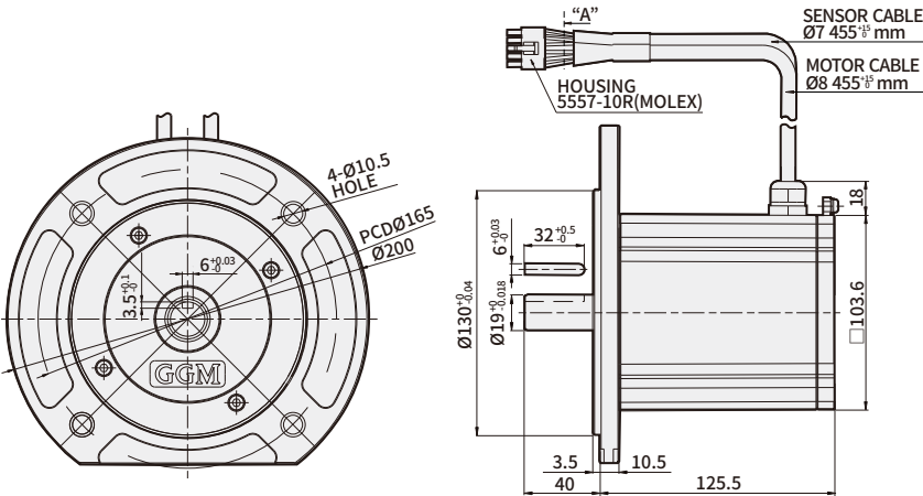
K20BK750NC Weight : 5.3Kg
