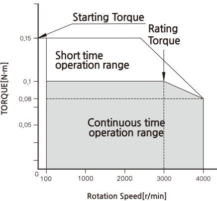
K10FS200NC / K10FH200NC
