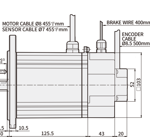
K16BK750NC-BE (Brake Encoder type) Weight : 5.7Kg
