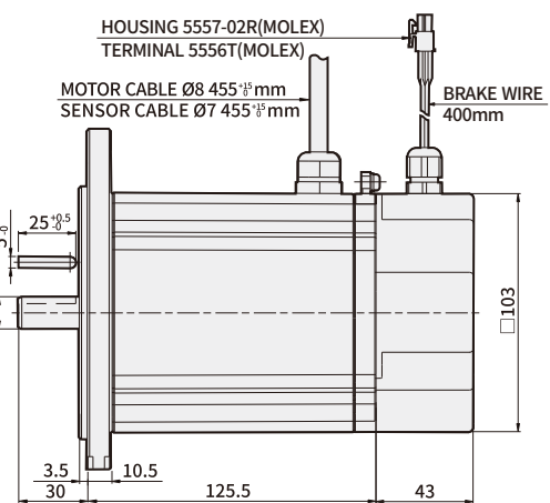
K16BK750NC-B (Brake type) Weight : 5.6Kg
