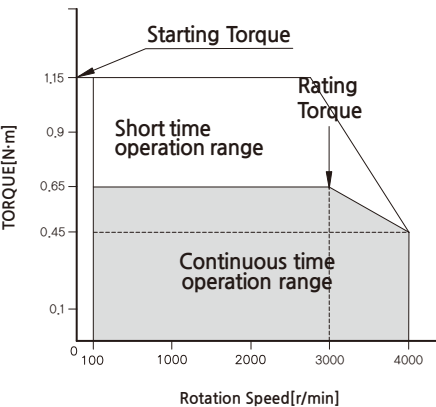
K10FS200NC / K10FH200NC
