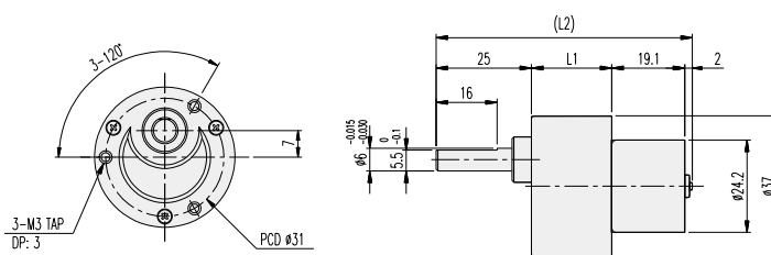
GEARHEAD LENGTH
