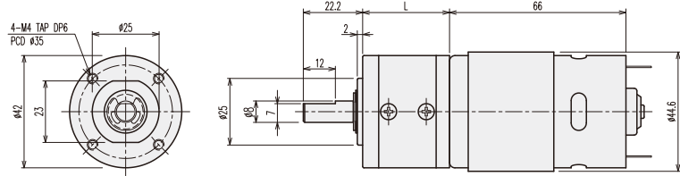
GEARHEAD LENGTH
