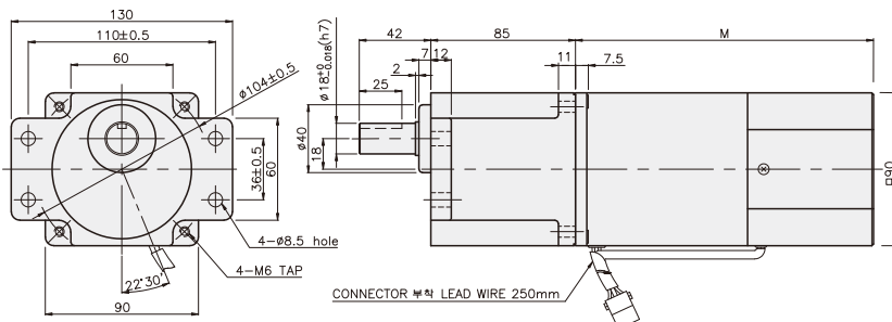
K9IP120F□-SU + K9P□BUF
