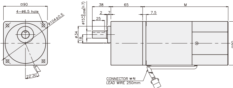
K9IP120F□-SU + K9P□B
