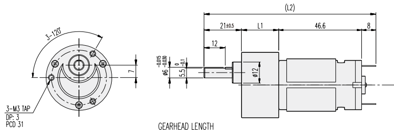
GEARHEAD LENGTH
