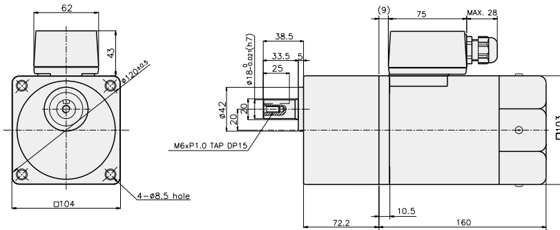
K10IH200F□-T5 + K10H□B
