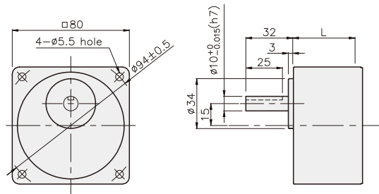
GEARHEAD K8G□B(C)
