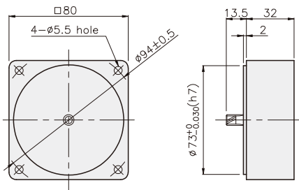
DECIMAL GEARHEAD K8G10BX
